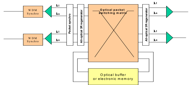
Figure 1 - Structure of an all-optical packet router
